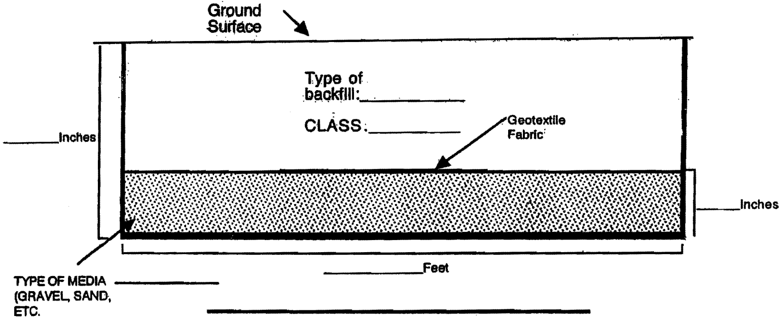
TYPICAL EXCAVATION - GREATER THAN 4' WIDTH - CROSS SECTION - NO SCALE
